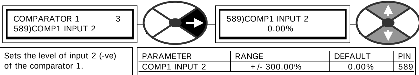
3.15.3 COMPARATOR 1/2/3/4 / Input 2 PIN 589/593/597/601
