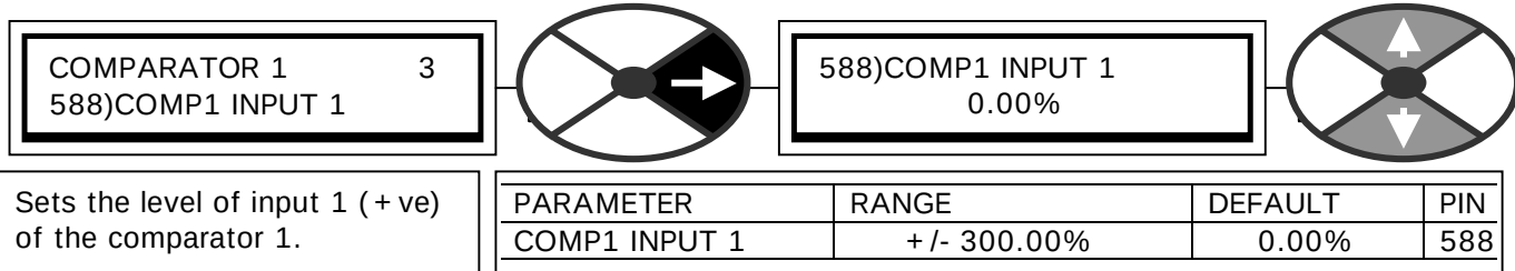
3.15.2 COMPARATOR 1/2/3/4 / Input 1 PIN 588/592/596/600
