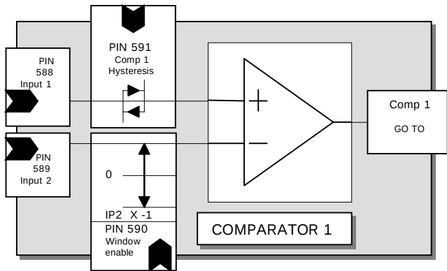
3.15.1 COMPARATOR 1 / Block diagram
